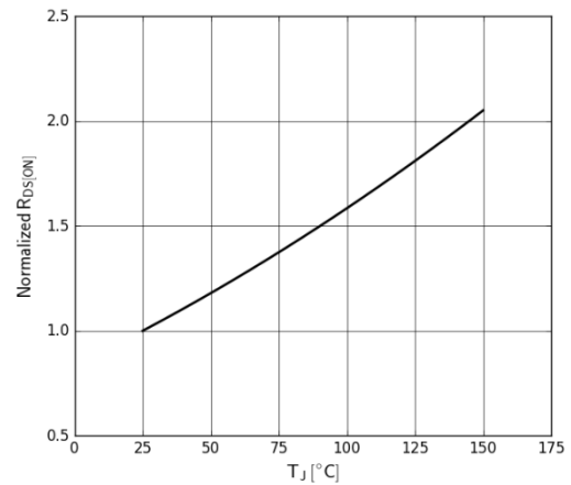
Figure 7. Normalized On-resistance
