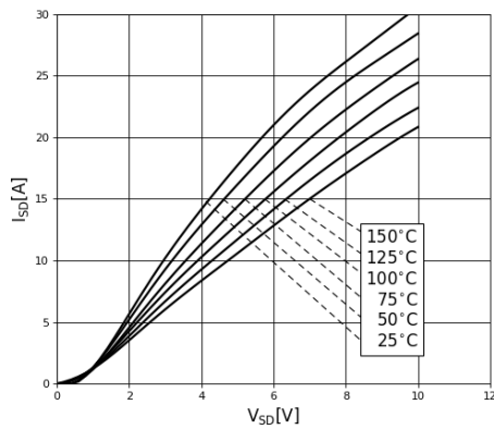
Figure 14. Forward Characteristics of Rev. Diode
