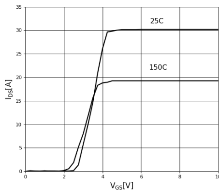
Figure 6. Typical Transfer Characteristics
