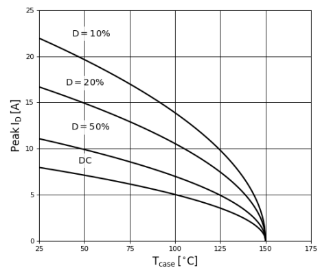
Figure 13. Current Derating
