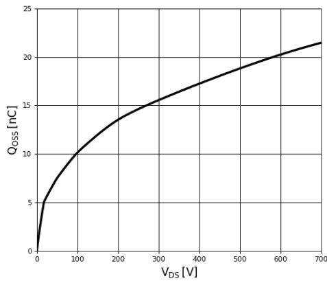
Figure 10. Typical QOSS
