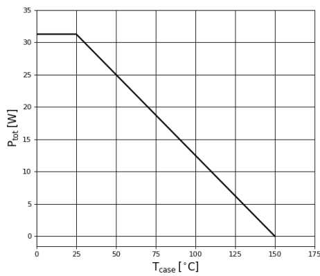
Figure 12. Power Dissipation
