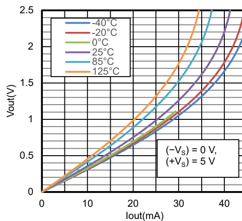
Figure 8. Output Voltage vs. Output Sinking Current, 5 V
