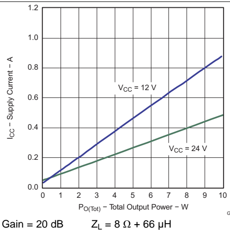
Figure 12. Supply Current vs Total Output Power
