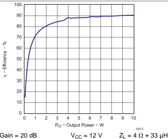
Figure 11. Efficiency vs Output Power
