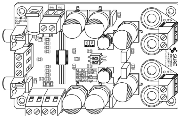
FIGURE 1-1 PRODUCT DIAGRAM
