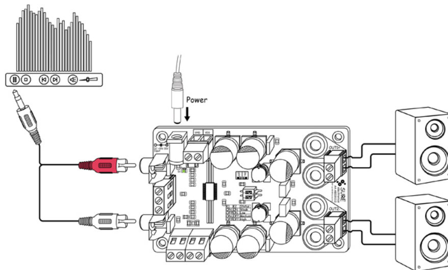
FIGURE 1-3 CONNECTION SCHEMATIC
