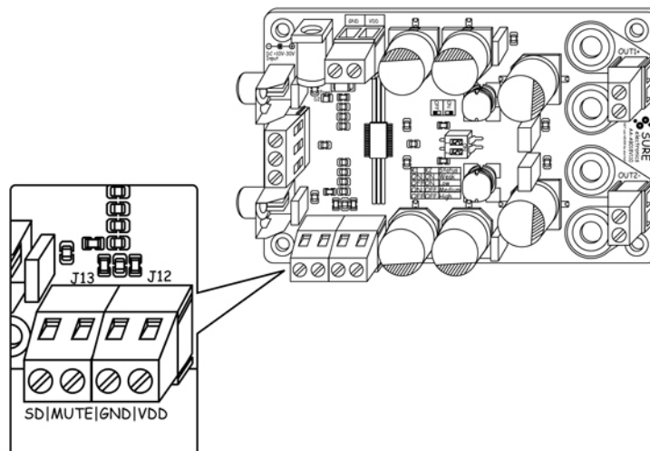
FIGURE 2-5 CONNECTION SCHEMATIC
