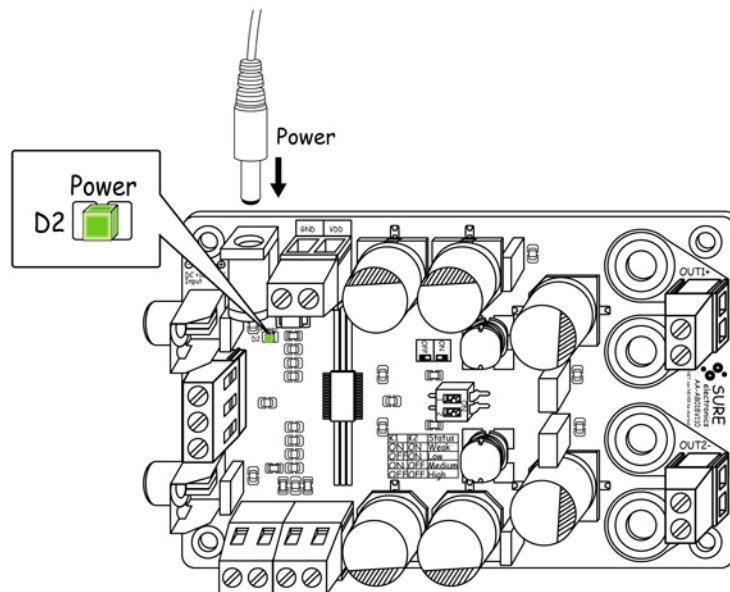
FIGURE 2-9 LED INDICATOR
