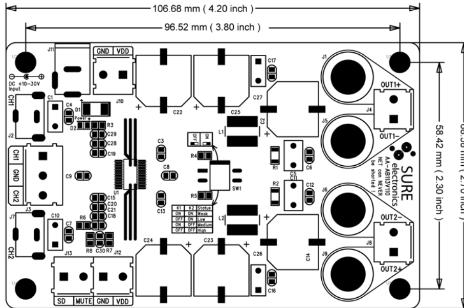
FIGURE 4-1 MECHANICAL DRAWING
