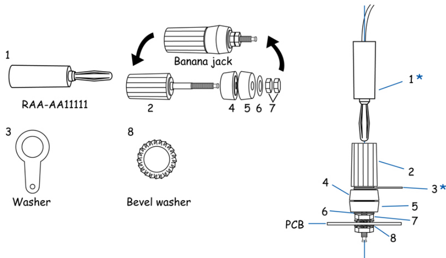
FIGURE 2-4 OUTPUT CONNECTION 2
