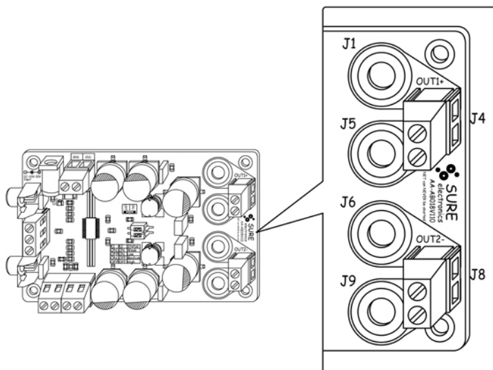
FIGURE 2-3 OUTPUT CONNECTION 1
