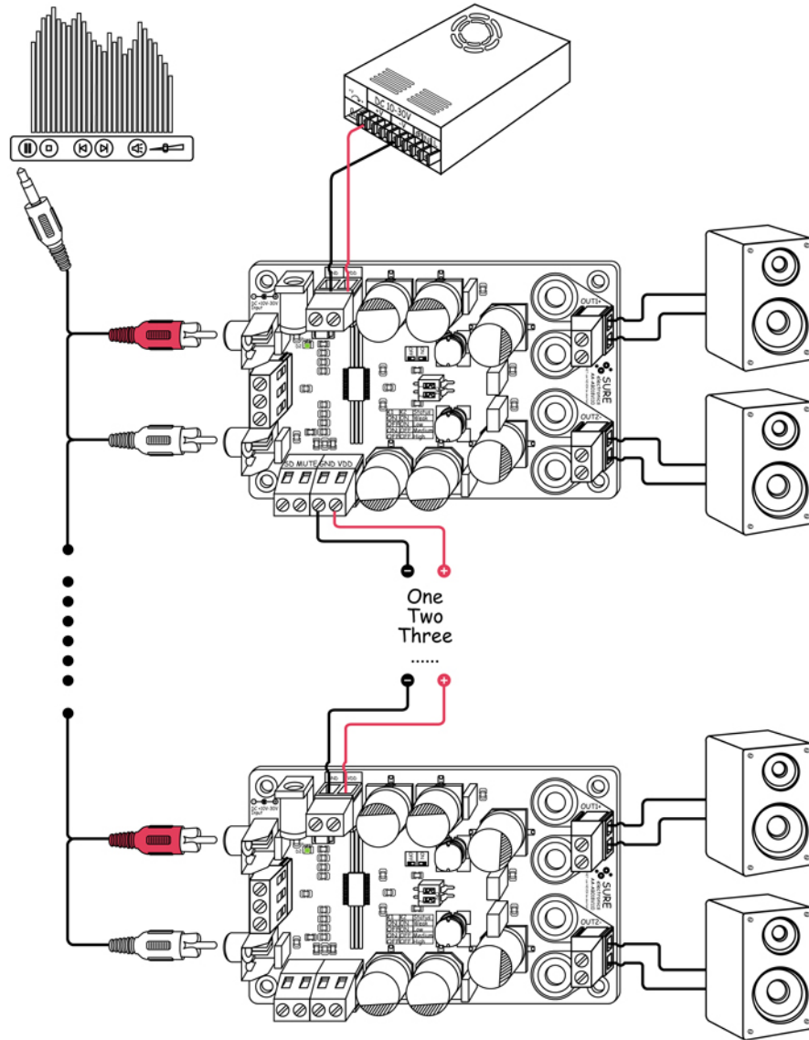
FIGURE 1-4 CASCADING SCHEMATIC
