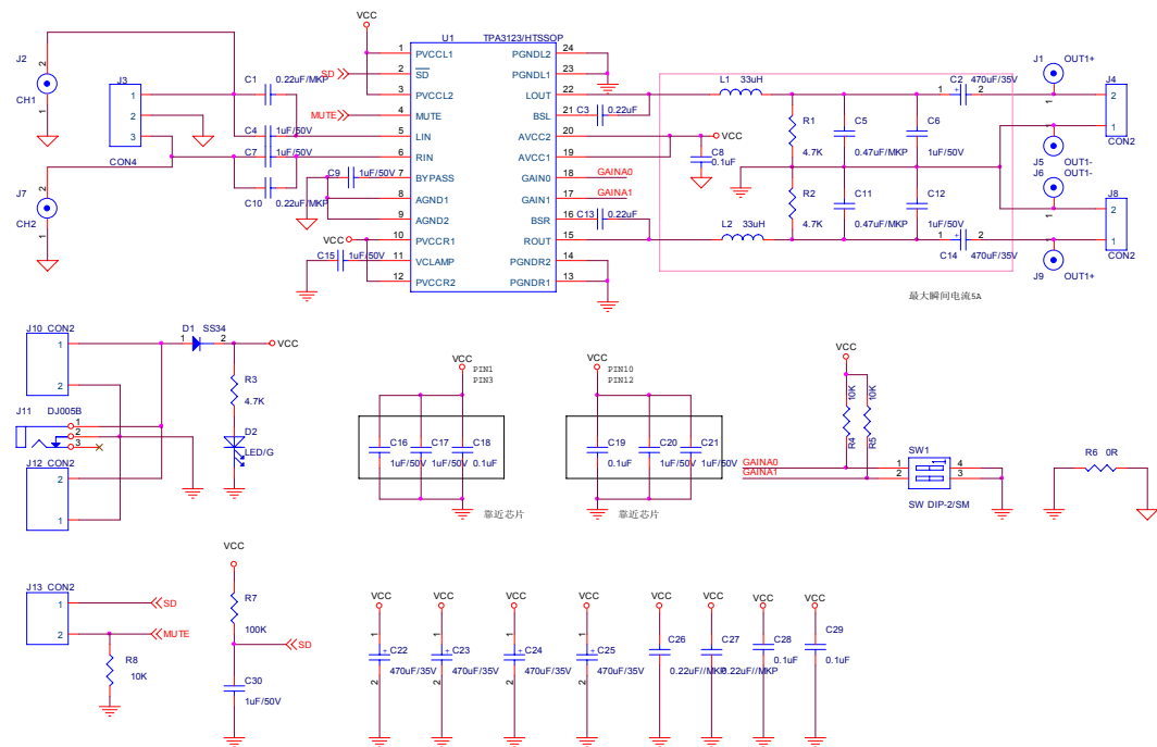
FIGURE 5-1 SCHEMATIC
