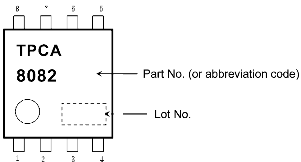
Fig. 7.1 Marking
