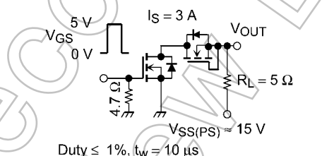
Fig. 7.2.1 Switching Time Test Circuit
