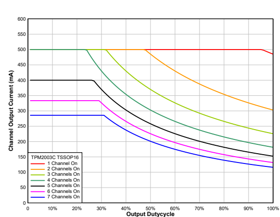
Figure 4. Output Current Capability vs. Duty Cycle
