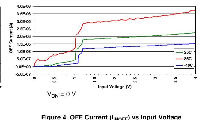
Figure 4. OFF Current ( I_{INOFF} ) vs Input Voltage
