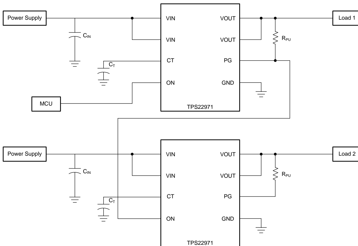
Figure 26. Power Sequencing
