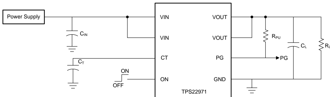
Figure 24. TPS22971 Test Circuit
