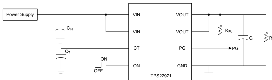
Figure 27. Typical Application Circuit
