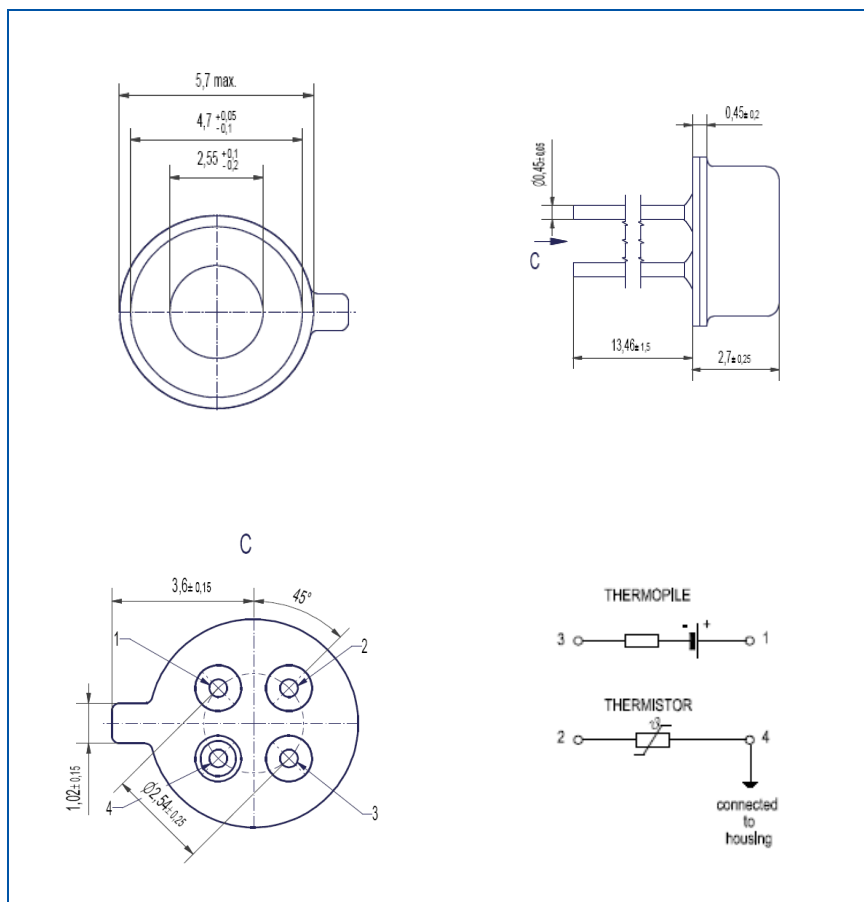
Figure 4: Mechanical Drawing of the TPS 232
