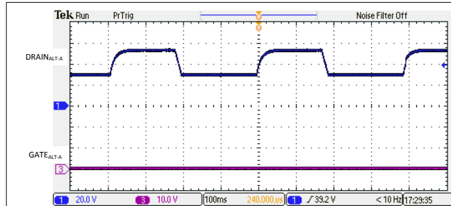
Figure 10-10. 2-Pair Open Circuit Detection Signature
