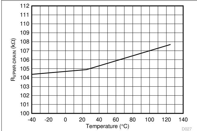
Figure 7-27. R OFF (VPWR to DRAIN) vs Temperature
