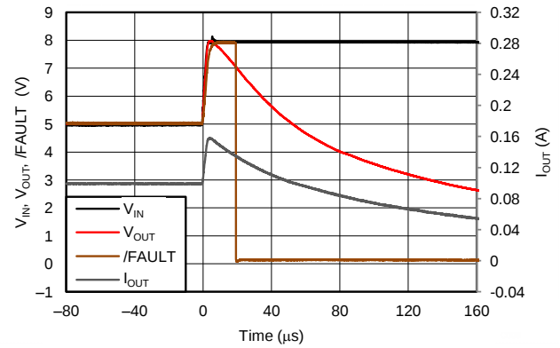
Figure 20. V_{IN} Step 5 V to 8 V With 4.7 \mu\text{F} // 100 \Omega
