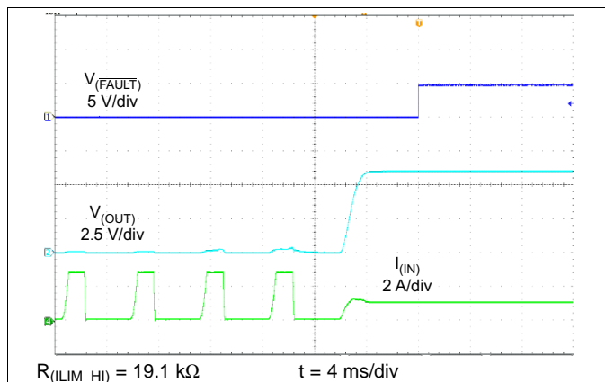
Figure 24. Short-Circuit to Full-Load Recovery
