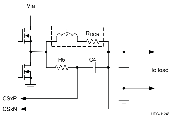
Figure 10. Current Sensing Using Inductor Resistance
