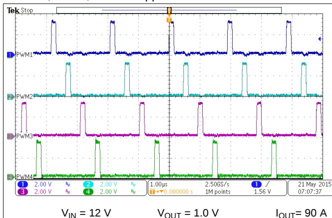
Figure 107. PWM Interleaving
