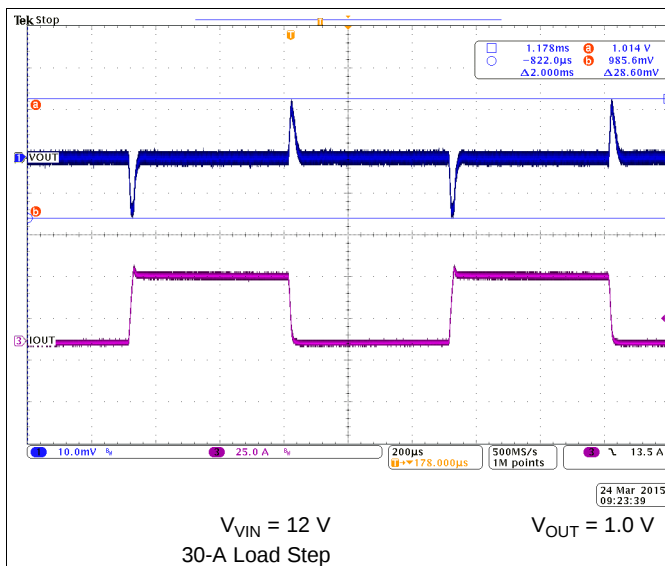
Figure 109. Transient Response
