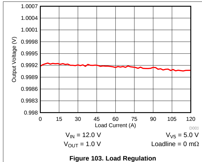
Figure 103. Load Regulation
