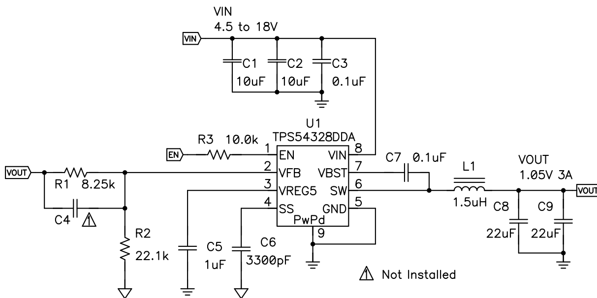
Figure 6. Schematic Diagram
