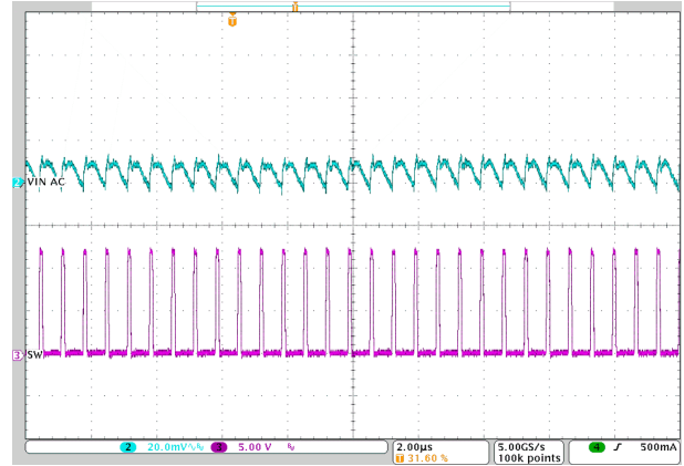
Figure 8-29. Input Ripple – No Load
