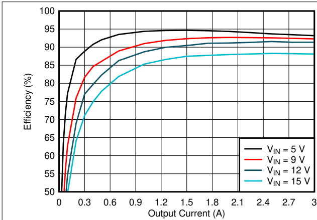
Figure 8-22. Efficiency
