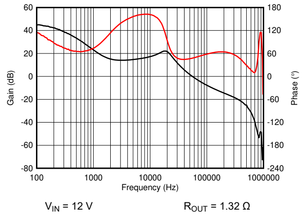
Figure 8-7. Bode Plot
