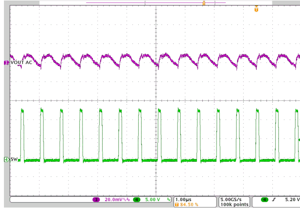
Figure 8-28. Output Ripple – 3-A Load
