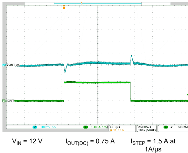
Figure 8-26. Load Transient
