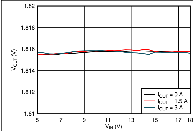
Figure 8-24. Line Regulation
