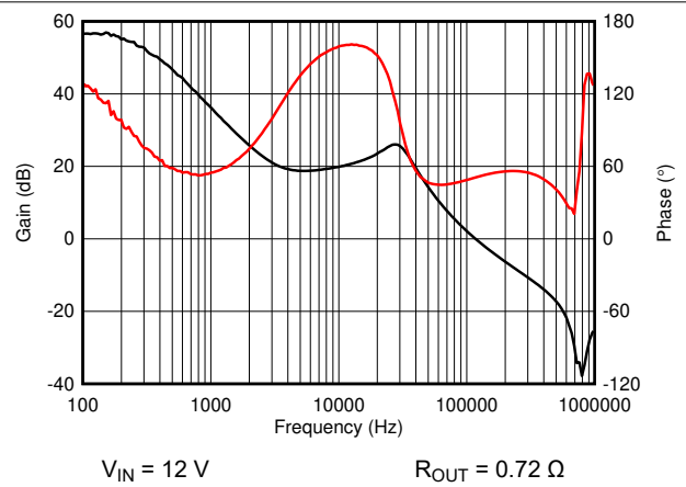
Figure 8-25. Bode Plot
