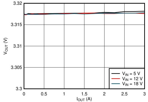
Figure 8-5. Load Regulation
