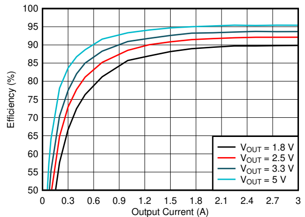
Efficiency at 12 V_{in} 1 MHz
