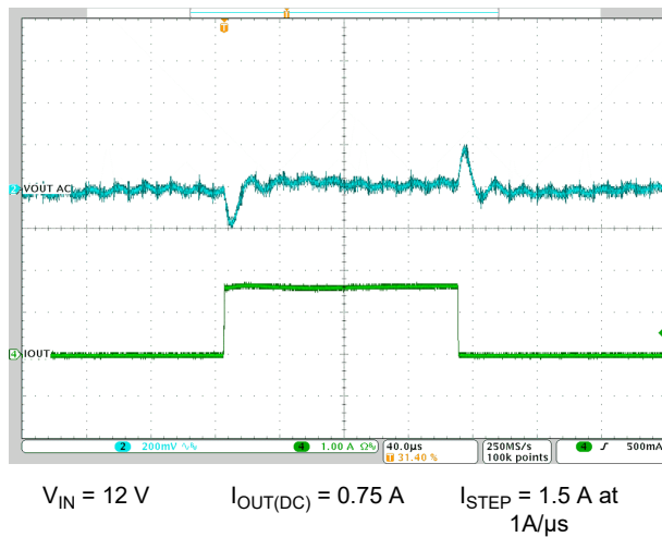
Figure 8-8. Load Transient
