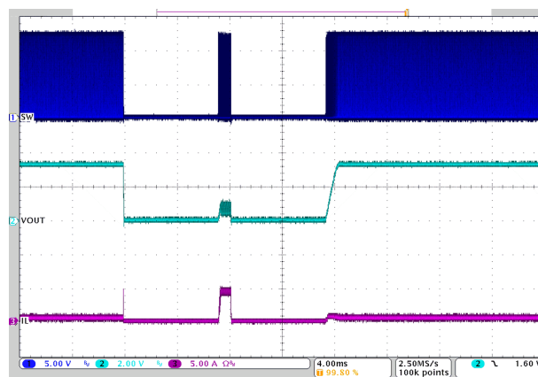
Figure 8-18. Overcurrent Protection – Overload
