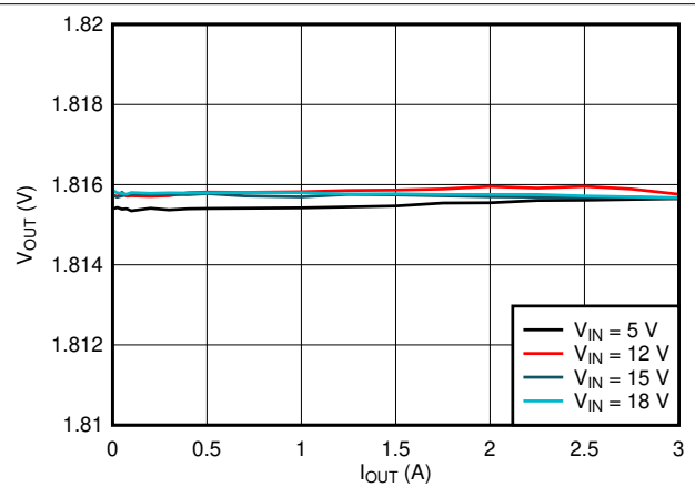
Figure 8-23. Load Regulation
