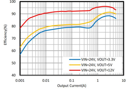
Figure 3. Efficiency vs Load Current, V_{in}=24V
