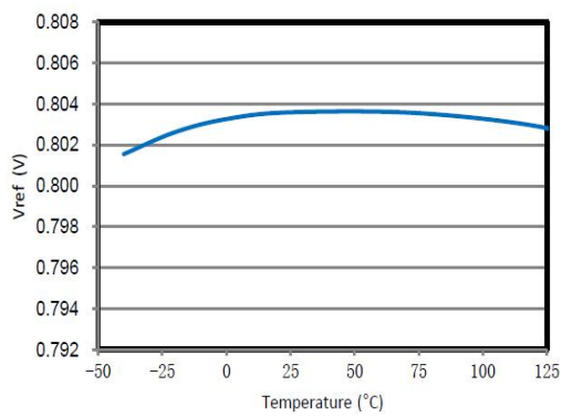
Figure 12. Reference Voltage vs Temperature
