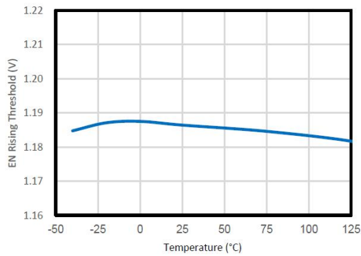
Figure 10. EN Threshold vs Temperature
