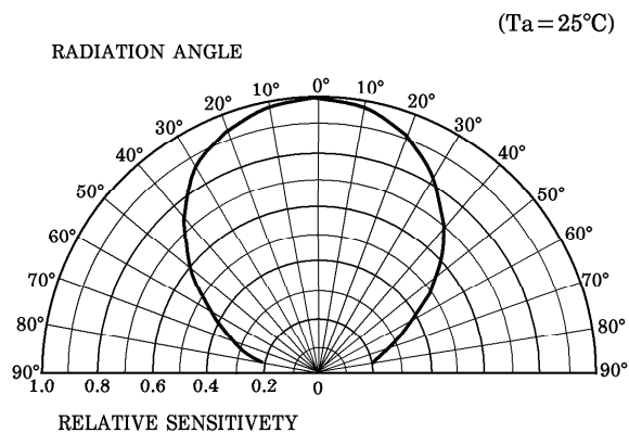
DECTIONAL SENSITIVITY CHARACTERISTIC (TYP.)
