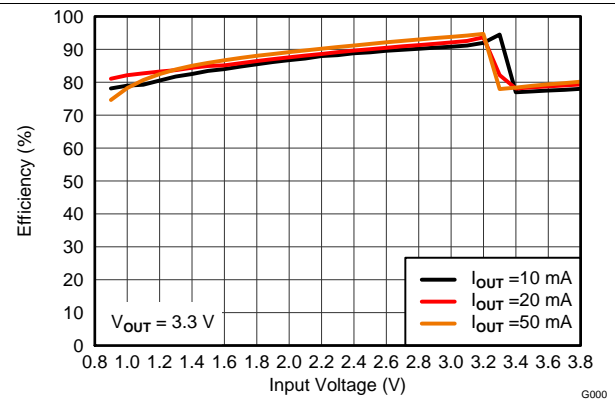
Figure 8. Efficiency vs Input Voltage
