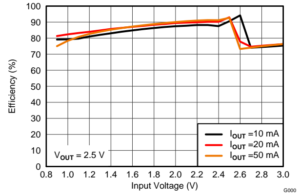
Figure 6. Efficiency vs Input Voltage
