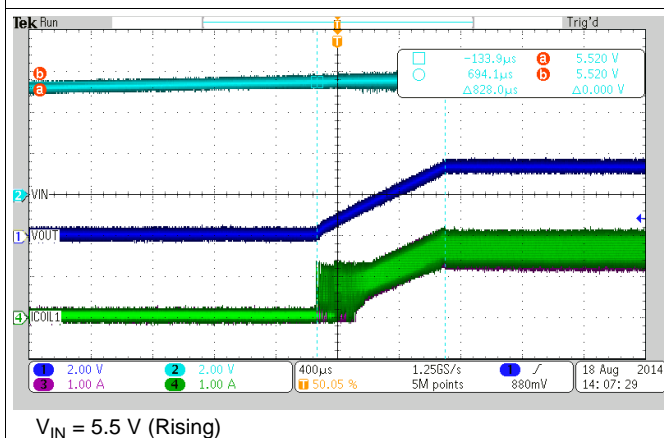
Figure 31. Accurate EN Threshold
