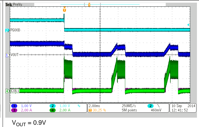
Figure 30. HICCUP at Short Circuit
