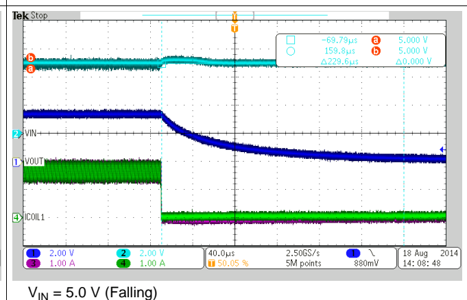
Figure 32. Accurate EN Threshold Showing V OUT
