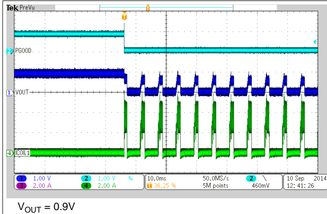
Figure 29. HICCUP at Short Circuit
