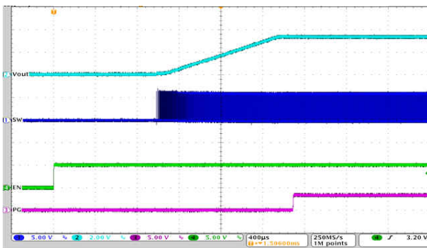
Figure 9-64. Start-Up Timing
