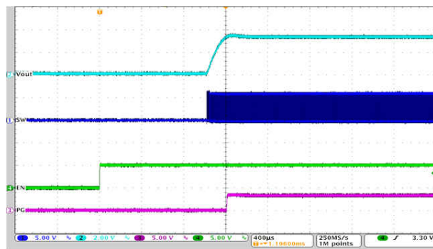
Figure 9-65. Start-Up Timing
