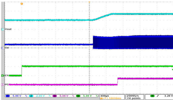
Figure 9-66. Start-Up Timing
