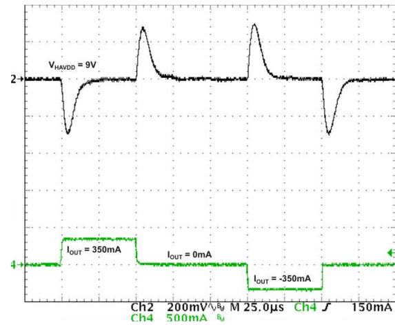
Figure 33. Buck 3 ( V_{HAVDD} ) PWM – Normal Load Source
