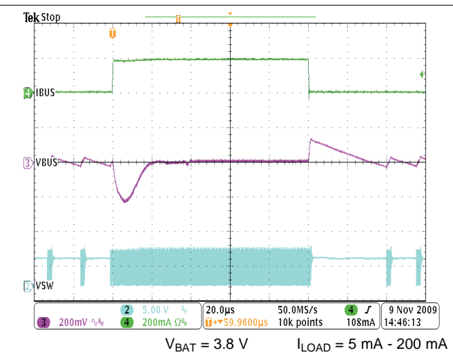
Figure 14. Transient Response
