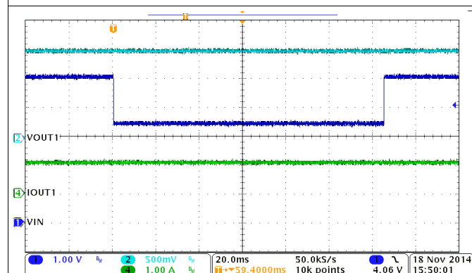
Figure 62. 180° Out-of-Phase
