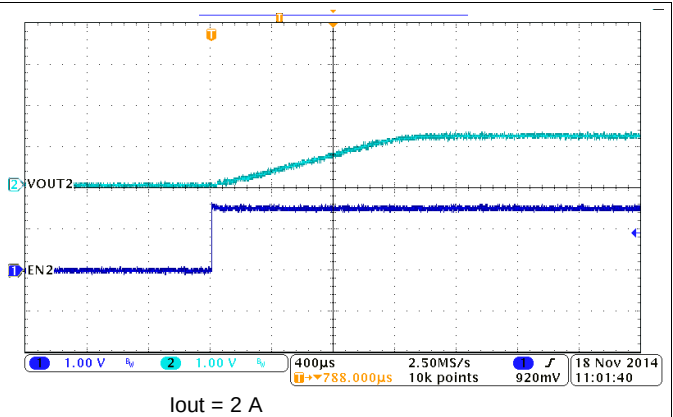
Figure 45. BUCK2, Soft-Start
