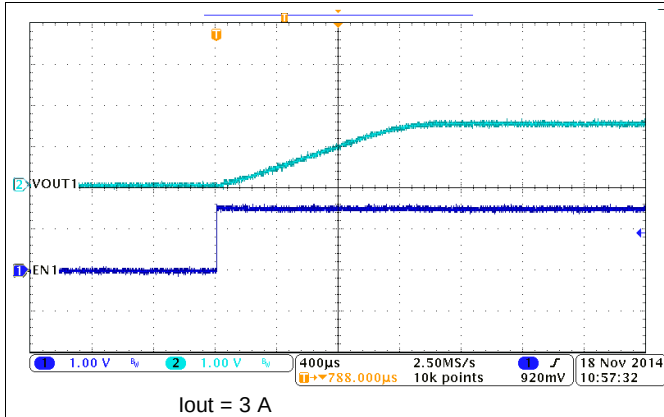
Figure 44. BUCK1, Soft-Start
