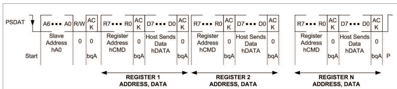
Figure 3-3. Power I 2 C Protocol
