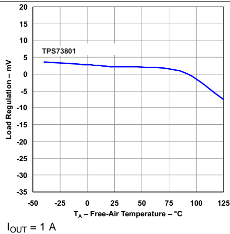
Figure 19. Load Regulation vs Temperature
