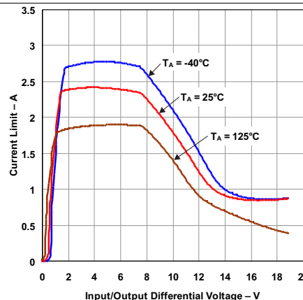
Figure 14. Current Limit vs Input/Output Differential Voltage
