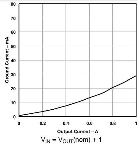
Figure 8. Ground Current vs Output Current
