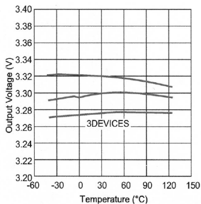
3.3V Output Voltage vs. Temperature
