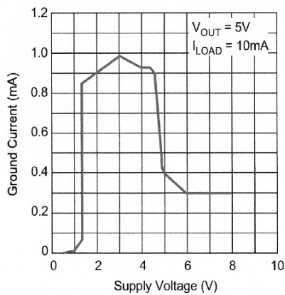
Ground Current vs. Supply Voltage
