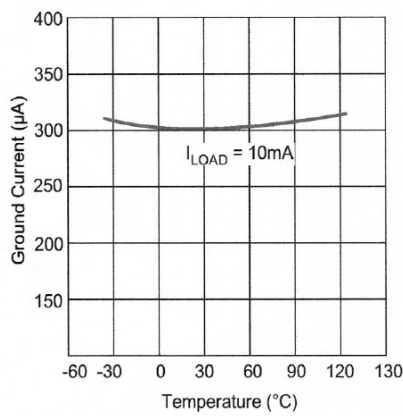
Ground Current vs. Temperature
