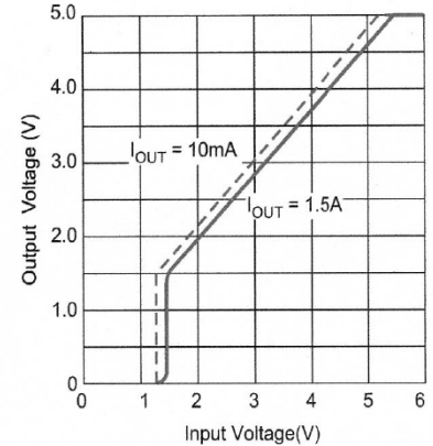
5.0V Dropout Characteristics
