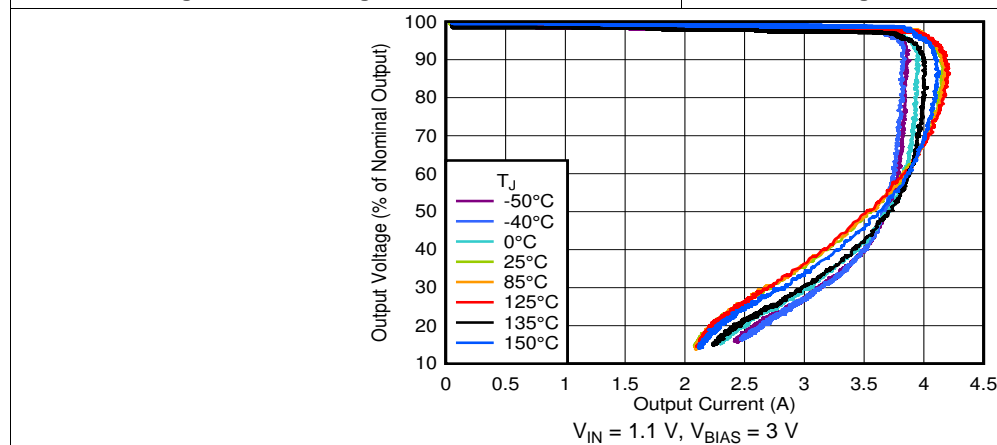
Figure 39. Foldback Current Limit vs Temperature
