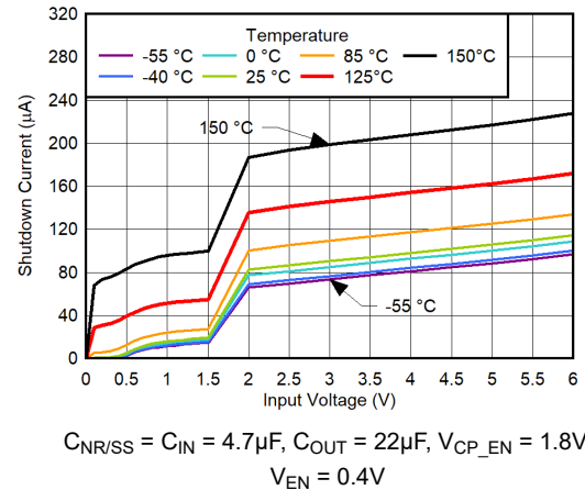
Figure 5-194. IN Pin Shutdown Current vs V_{IN} for V_{OUT} = 0.5V , V_{BIAS} = 3V , CP Enabled
