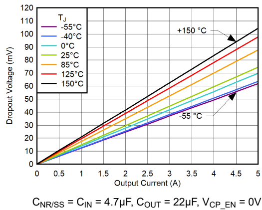
Figure 5-71. Dropout Voltage vs I_{OUT} for CP Disabled, V_{IN} = 0.7V , V_{BIAS} = 3.9V
