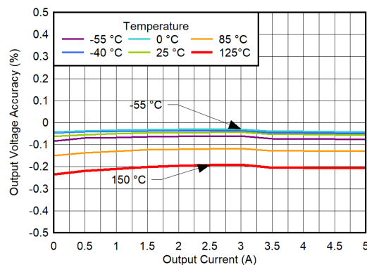
Figure 5-114. Output Voltage Accuracy vs I_{OUT} for V_{OUT} = 0.5V , V_{BIAS} = 3V , CP Enabled
