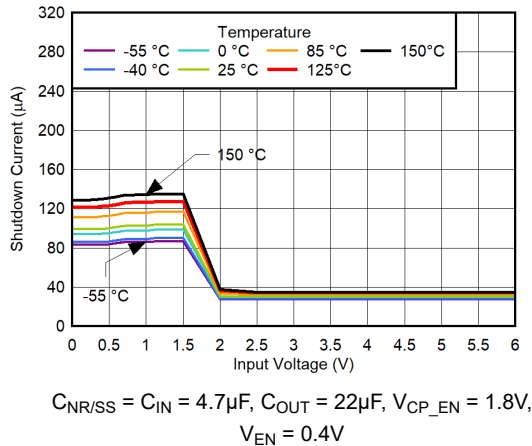
Figure 5-193. BIAS Pin Shutdown Current vs V_{IN} for V_{OUT} = 0.5V , V_{BIAS} = 3V , CP Enabled
