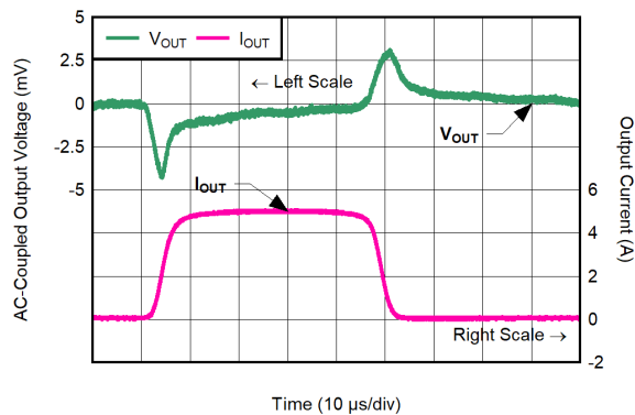
Figure 5-37. Load Transient for V_{OUT} = 0.5V , I_{OUT} = 100mA to 5 A, CP Disabled, SR = 0.5A/\mu s
