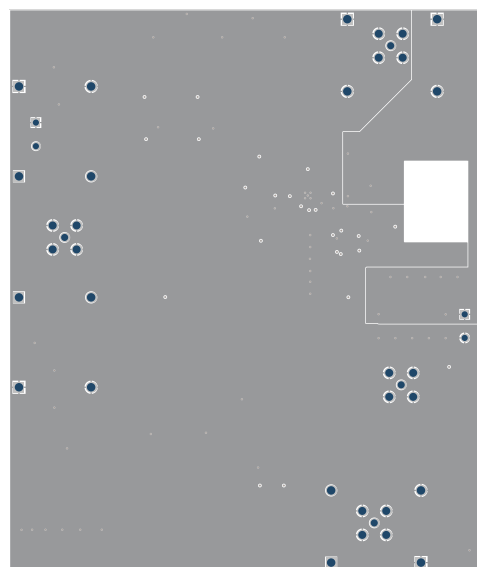
Figure 7-28. Layer 5 Routing
