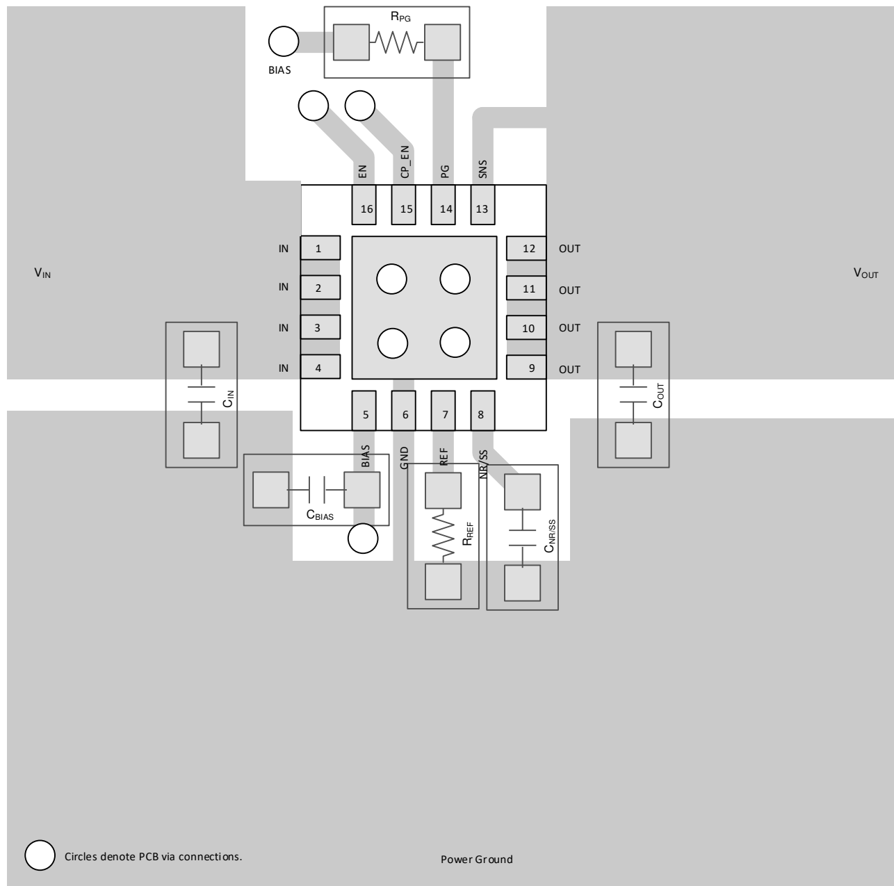
Figure 7-38. Recommended Layout
