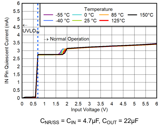
Figure 5-148. IN Pin Quiescent Current vs V_{IN} for V_{OUT} = 0.5V , V_{BIAS} = 11V , CP Disabled
