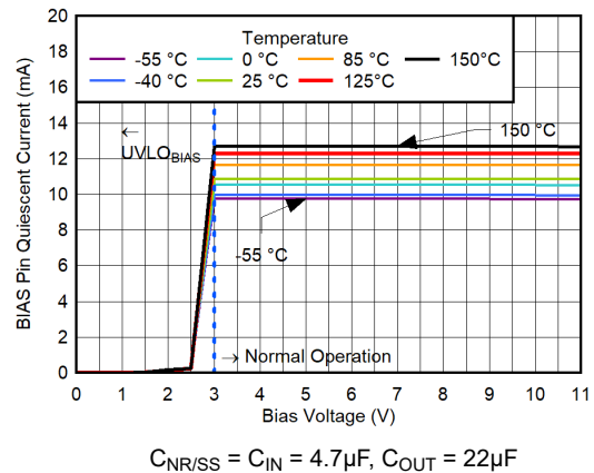
Figure 5-162. BIAS Pin Quiescent Current vs V_{BIAS} for V_{OUT} = 0.5V , V_{IN} = 0.7V , CP Enabled, I_{OUT} = 0A
