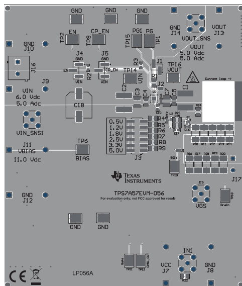
Figure 7-23. Top Assembly Layer and Silkscreen
