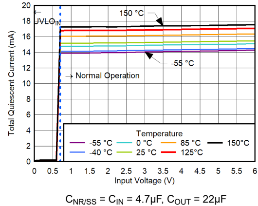
Figure 5-160. Total Quiescent Current vs V_{IN} for V_{OUT} = 0.5V , V_{BIAS} = 11V , CP Enabled, I_{OUT} = 0A
