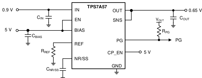
Figure 7-8. Typical Circuit
