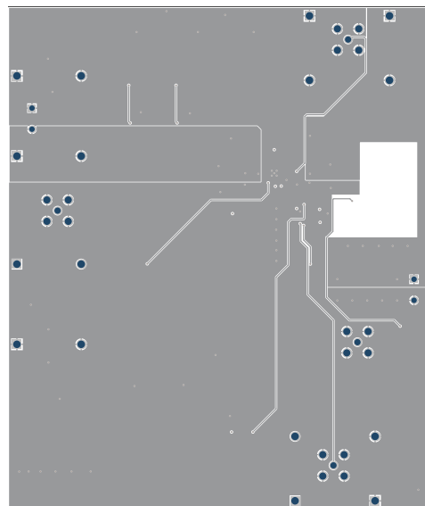
Figure 7-26. Layer 3 Routing
