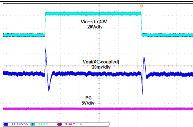
Figure 11. Line Transient Response, I_L = 1 mA, 1 V/ \mu s
