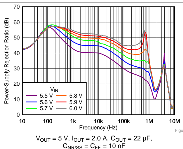
Figure 4. PSRR vs Frequency and Input Voltage
