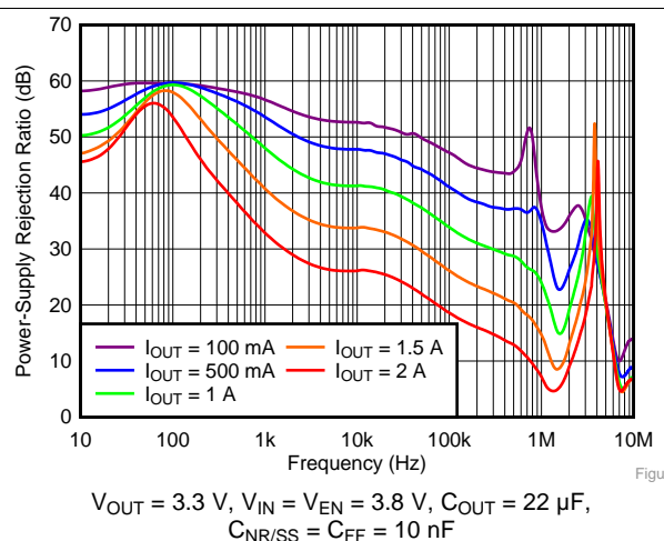
Figure 6. PSRR vs Frequency and Output Current
