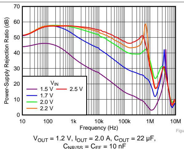
Figure 2. PSRR vs Frequency and Input Voltage
