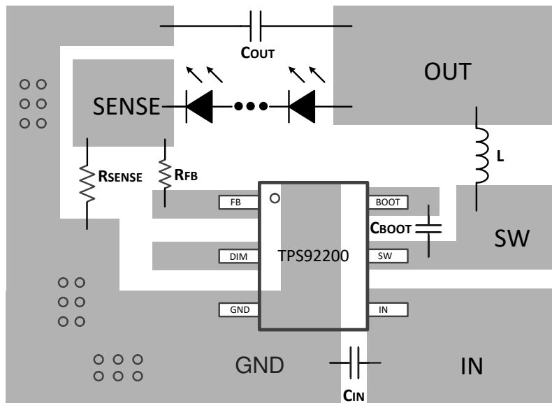
Figure 59. Layout Example
