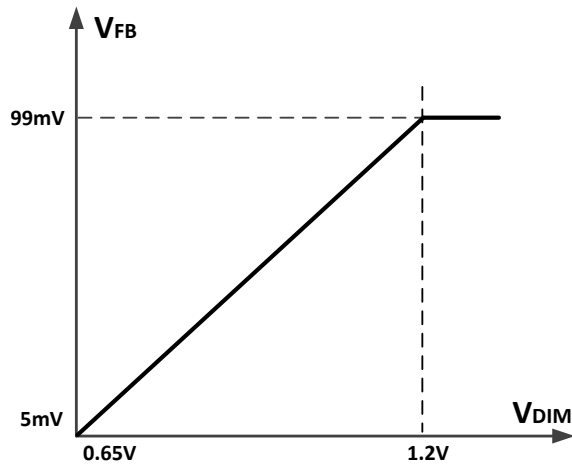
Figure 19. TPS92200D1 Analog Dimming
