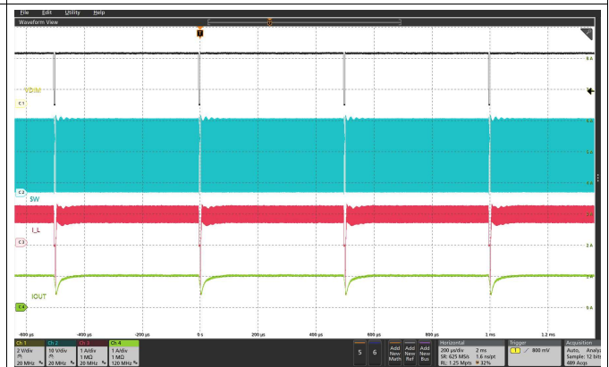
Black: DIM, Blue: SW, Red: Inductor Current, Green: LED Current Figure 45. LED PWM Dimming at 99% Duty Cycle and 2 kHz
