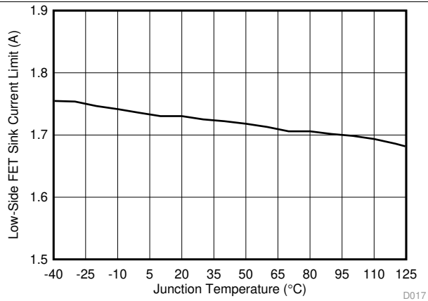
Figure 14. Low-Side FET Sink Current Limit vs. Junction Temperature
