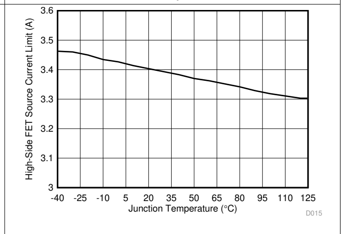
Figure 12. High-Side FET Source Current Limit vs. Junction Temperature
