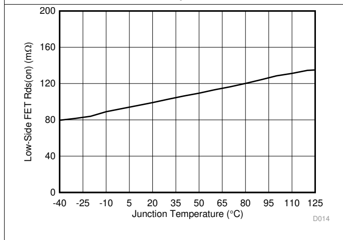
Figure 11. Low-Side FET On Resistance vs. Junction Temperature
