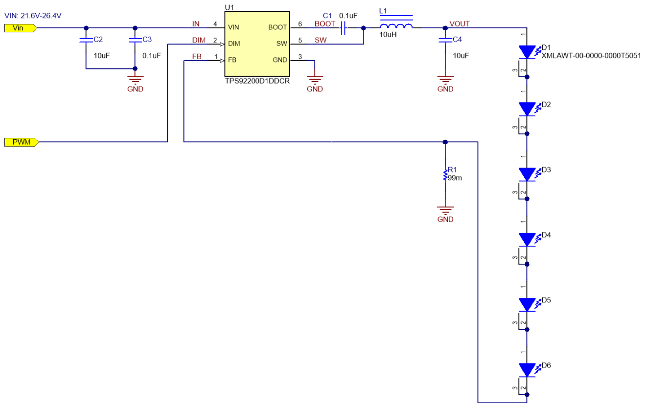
Figure 33. 24-VIN, 1-A, 6-piece WLED, PWM Dimming Reference Design
