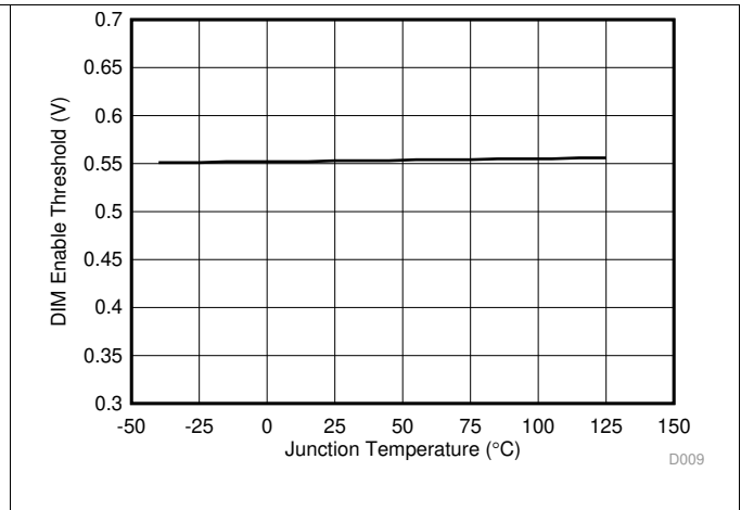
Figure 8. DIM Enable Threshold vs. Junction Temperature
