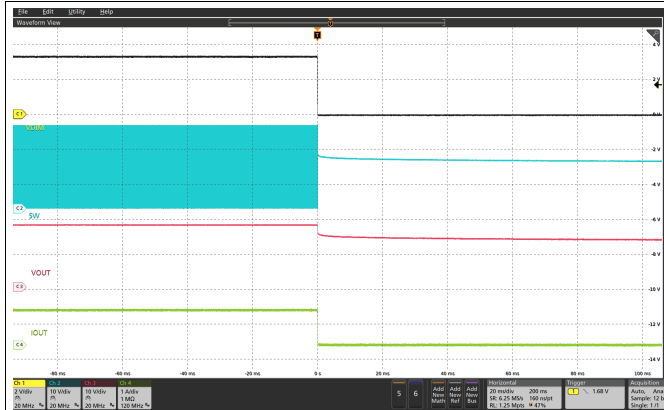
Black: DIM, Blue: SW, Red: VOUT, Green: LED Current Figure 40. Shutdown at 100% Duty Cycle and 500 Hz
