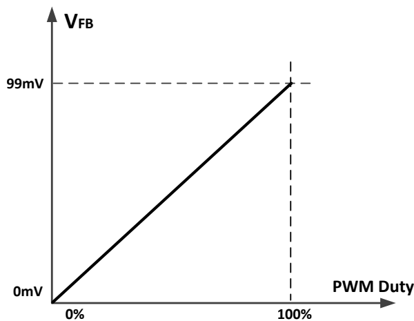
Figure 20. TPS92200D2 Analog Dimming
