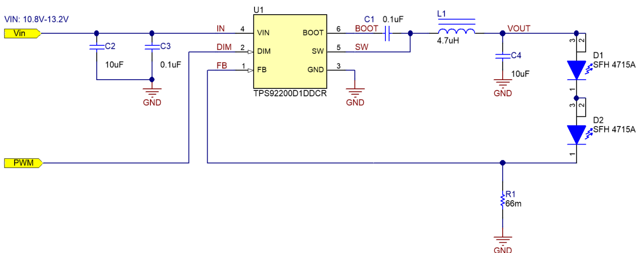
Figure 21. 12-VIN, 1.5-A, 2-piece IR LED, Analog Dimming Reference Design
