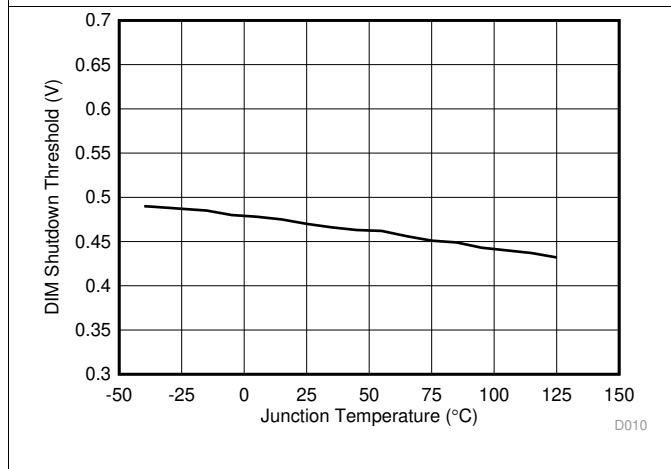
Figure 9. DIM Shutdown Threshold vs. Junction Temperature
