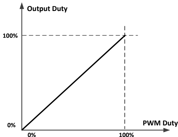
Figure 18. TPS92200D1 PWM Dimming
