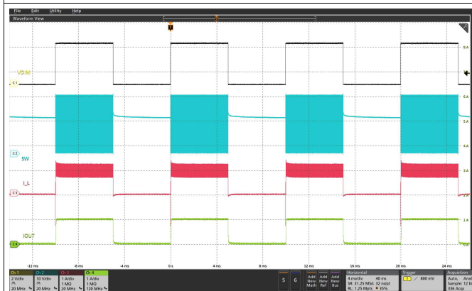
Black: DIM, Blue: SW, Red: Inductor Current, Green: LED Current Figure 42. LED PWM Dimming at 50% Duty Cycle and 200 Hz
