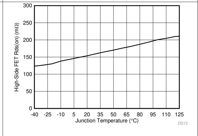
Figure 10. High-side FET On Resistance vs. Junction Temperature
