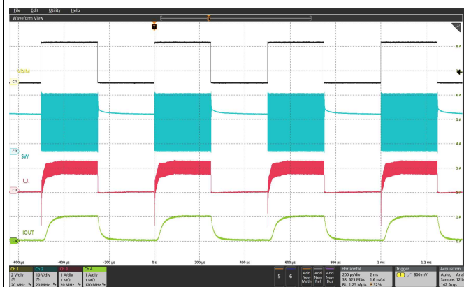
Black: DIM, Blue: SW, Red: Inductor Current, Green: LED Current Figure 44. LED PWM Dimming at 50% Duty Cycle and 2 kHz
