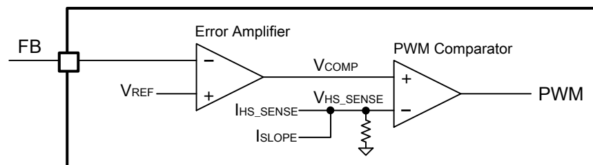
Figure 17. Error Amplifier and PWM Comparator
