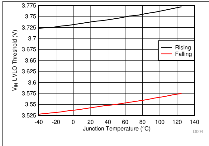
Figure 7. VIN UVLO Threshold vs. Junction Temperature
