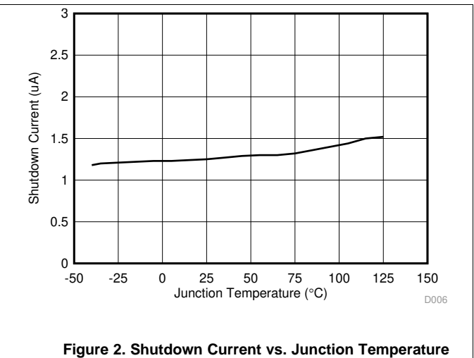
Figure 2. Shutdown Current vs. Junction Temperature
