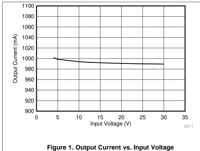
Figure 1. Output Current vs. Input Voltage
