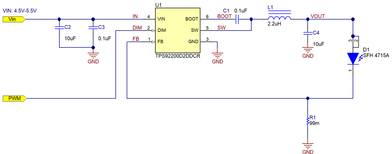
Figure 46. 5-VIN, 1-A, 1-piece IR LED, Analog Dimming Reference Design
