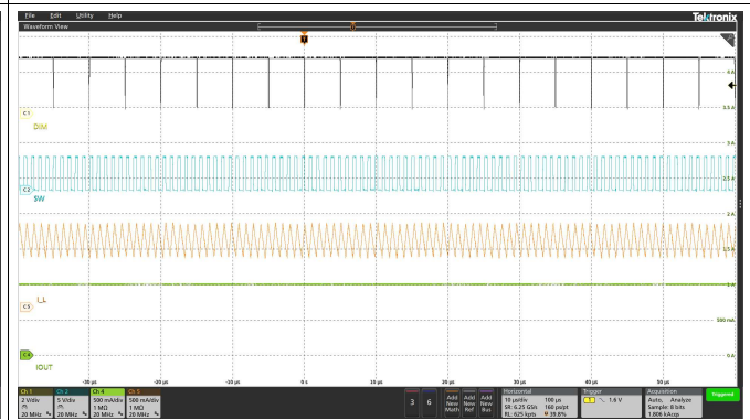
Figure 56. LED Analog Dimming at 1% Duty Cycle and 200 kHz
