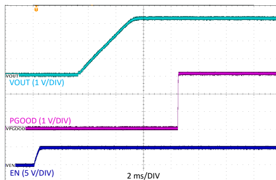
Figure 8-4. Enable Start-Up V_{IN} = 24\text{ V} , V_{OUT} = 3.3\text{ V} , I_{OUT} = 2.5\text{ A} I_{OUT} = 1.5\text{ A}
