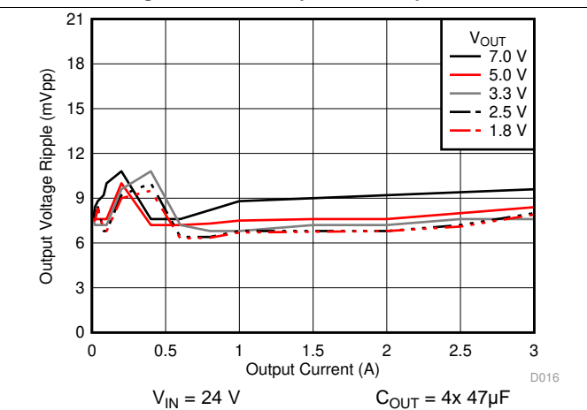
Figure 16. Voltage Ripple versus Output Current
