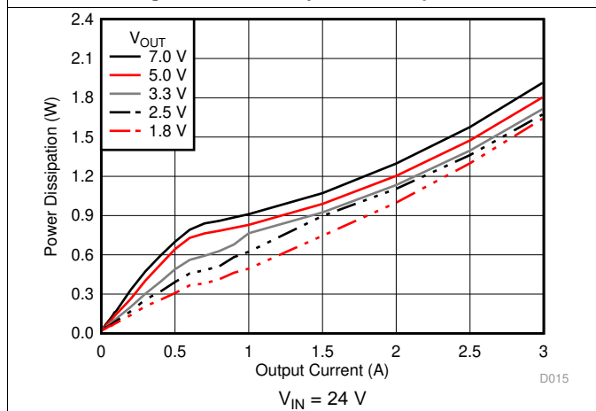
Figure 15. Power Dissipation versus Output Current
