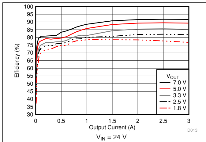
Figure 13. Efficiency versus Output Current
