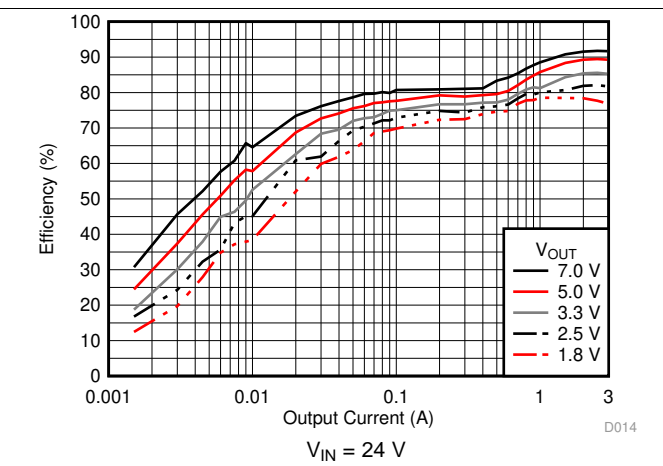
Figure 14. Efficiency versus Output Current
