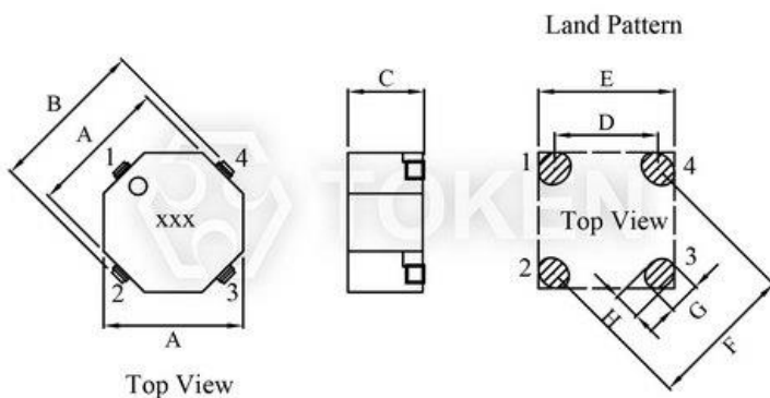
Low EMI Toroidal (TPSTX-2P/2S/4P/4S) Dimensions
