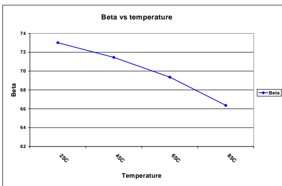
Beta versus Junction Temperature
