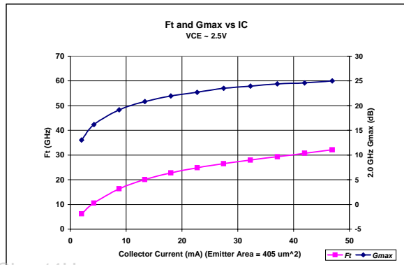
Ft and Gmax versus Collector Current
