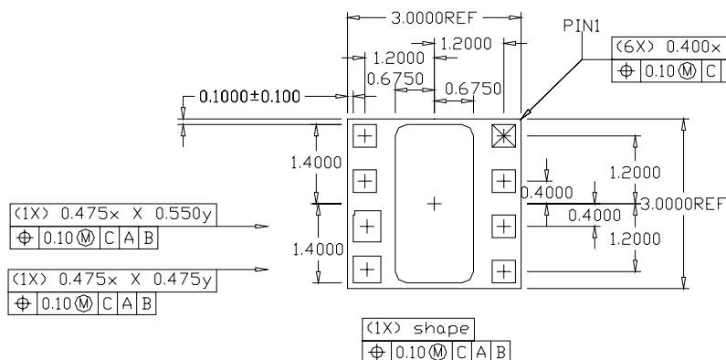
Figure 7: Package Drawing Information (Bottom View)
