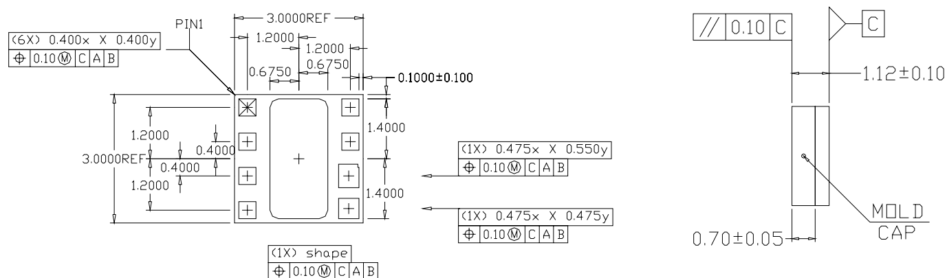
Figure 6: Package Drawing Information: Right (Top View) / Left (Side View)
