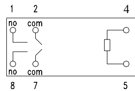
Form A
