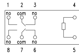
Form C
