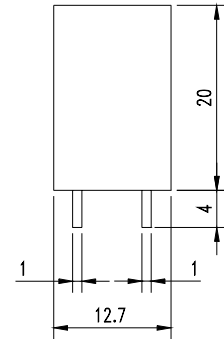
Terminal Arrangement/ Internal Connections (Bottom view)
