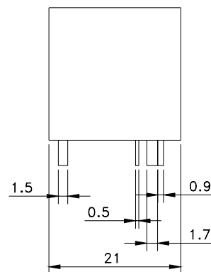
Terminal Arrangement/ Internal Connects (Bottom view)
