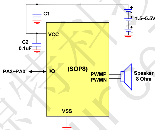
Figure 4. PWM Applications circuit
