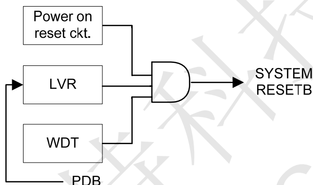
Figure 3: Reset structure
