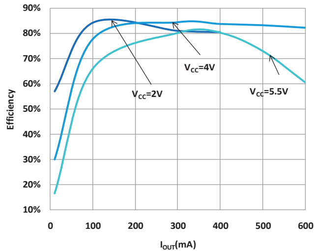
Fig.9 Efficiency vs. Output Current ( V_{OUT} = 0.8V )
