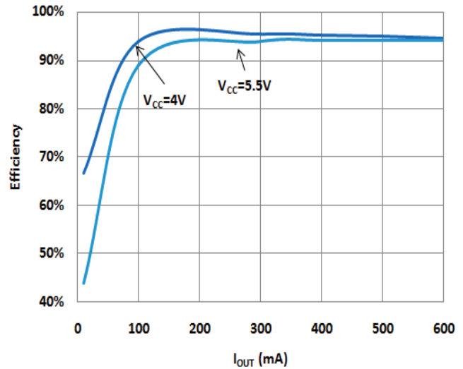
Fig.8 Efficiency vs. Output Current ( V_{OUT} = 3.3V )
