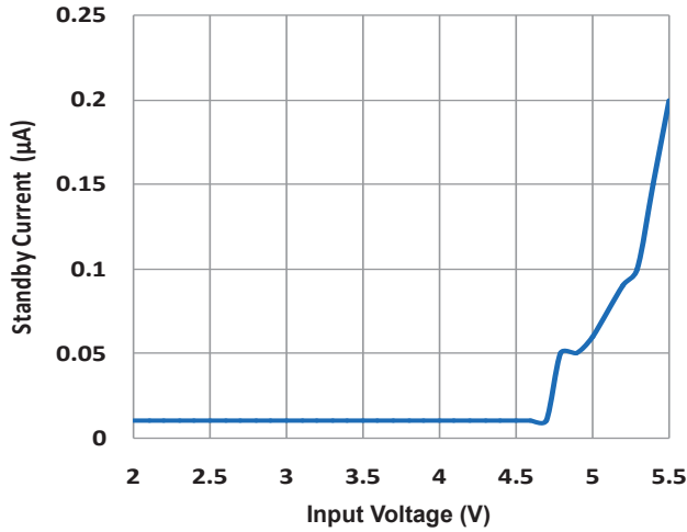
Fig.11 Standby Current vs. Input Voltage
