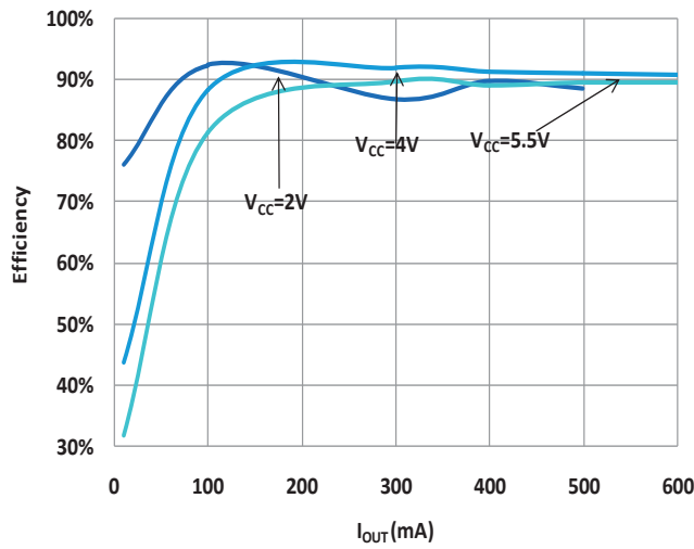
Fig.7 Efficiency vs. Output Current ( V_{OUT} = 1.8V )
