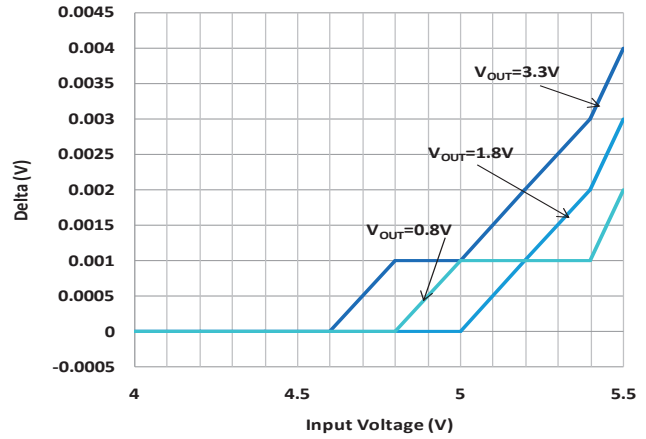
Fig.6 Line Regulation ( I_{OUT} = 300mA )
