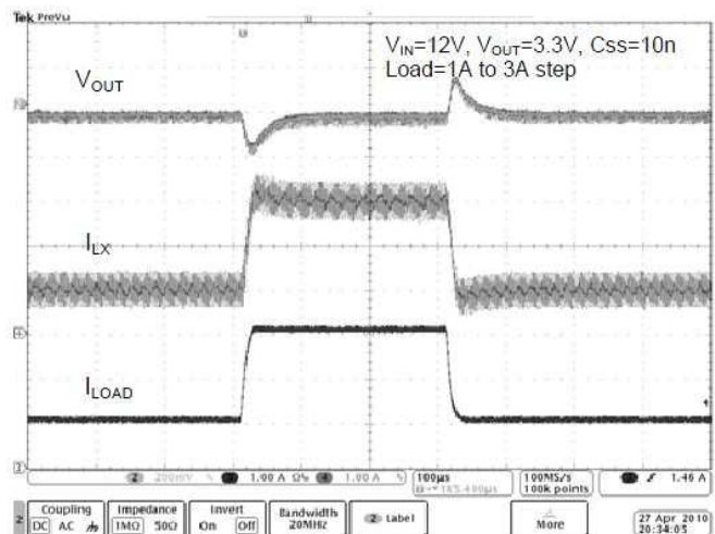
Figure 6. Load Transient
