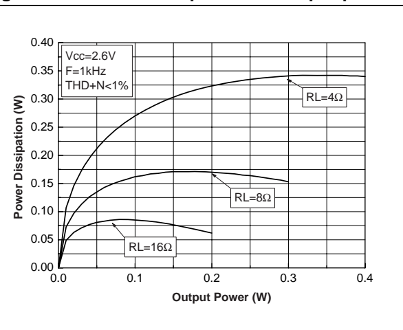
Figure 31. Power dissipation vs. output power
