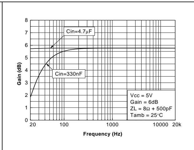
Figure 53. Frequency response
