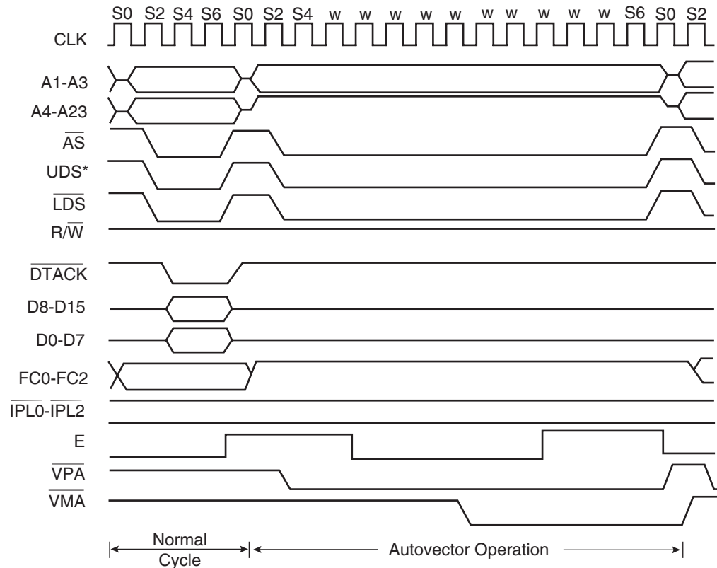
Figure 2-16. Autovector Operation Timing Diagram
