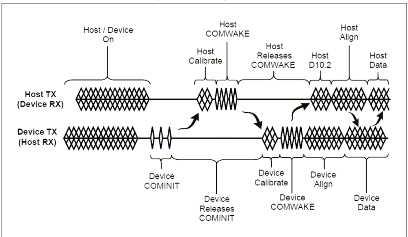
Figure 6 : cominit sequence
