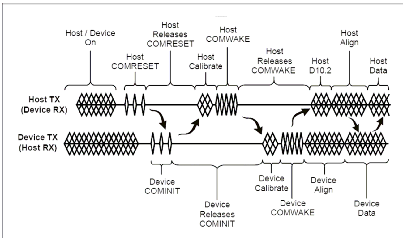
Figure 5 : comreset sequence
