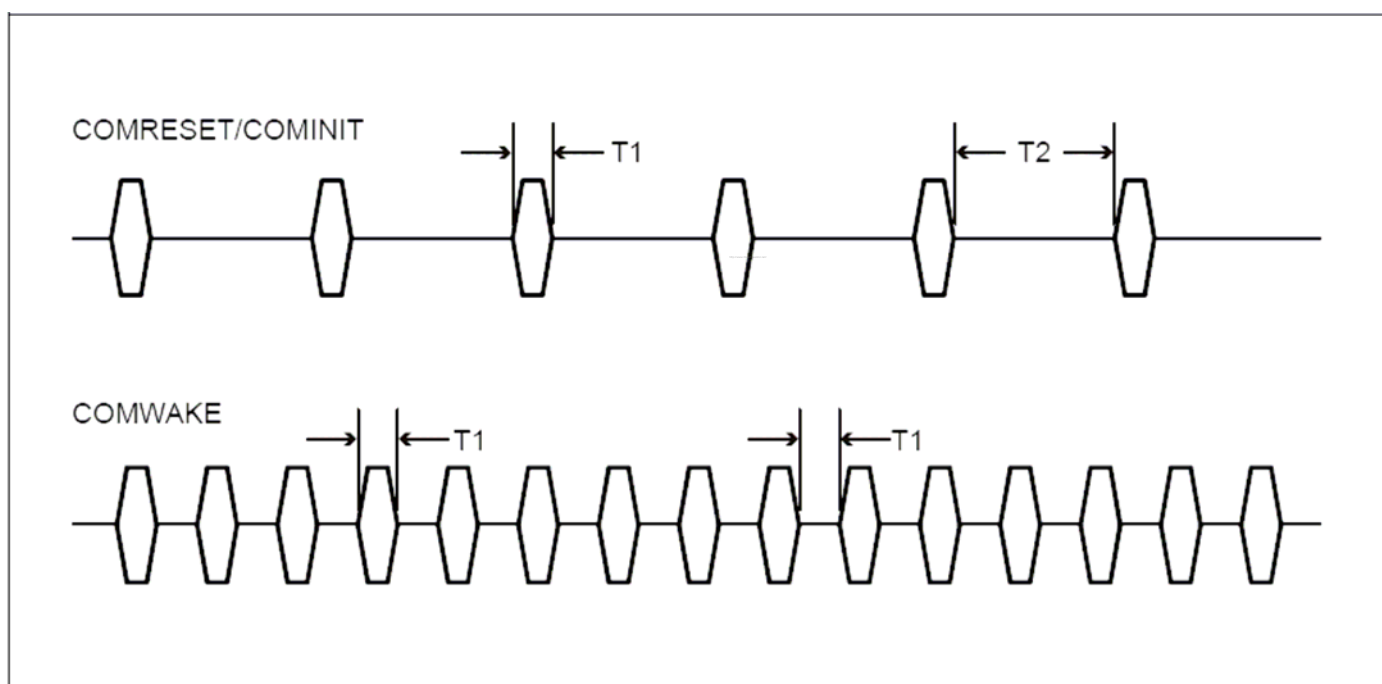
Figure 4 : OOB signals
