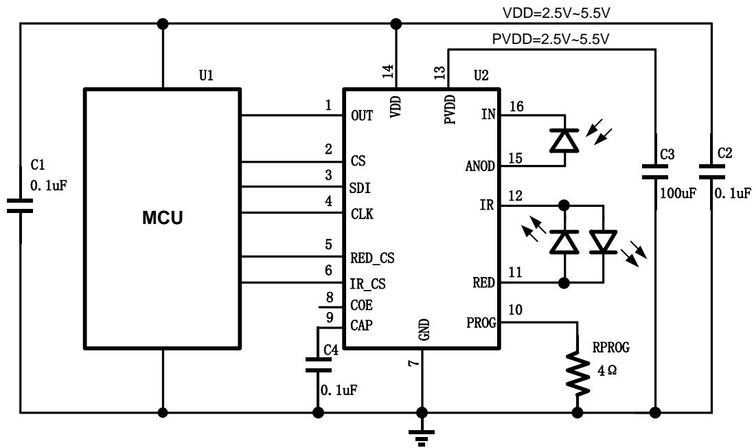
Figure 3. Typical Application of TS9517 in TSSOP16 Package
