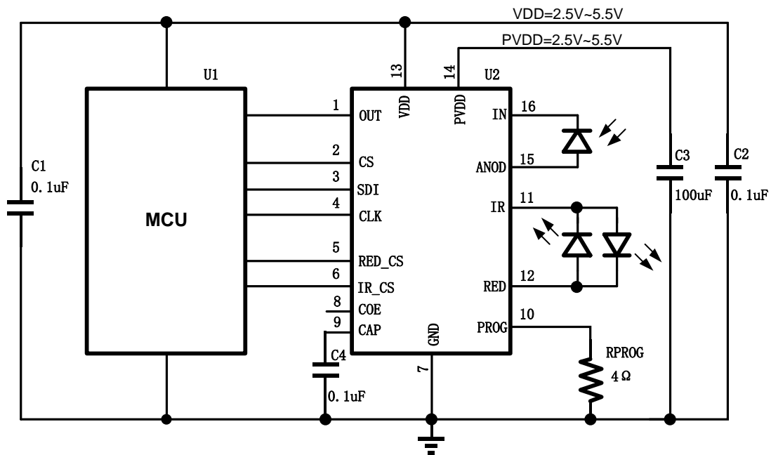
Figure 4. Typical Application of TS9517 in QFN16 Package
