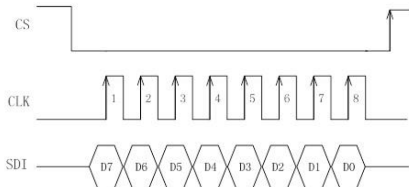
Figure 2. SPI timing diagram
