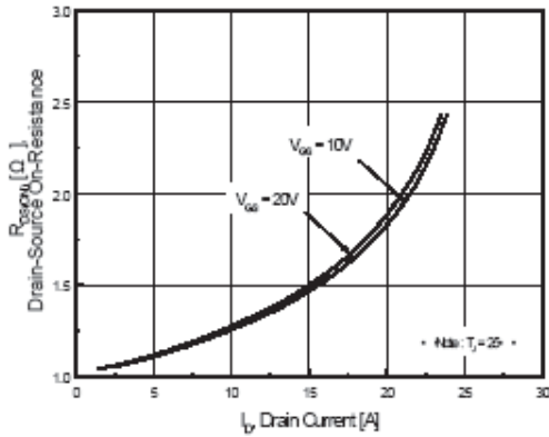
Figure 3. On-Resistance Variation
