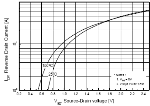
Figure 4. Body Diode Forward Voltage
