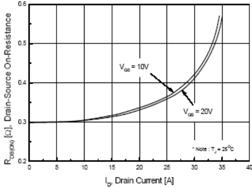
Figure 3. On-Resistance Variation
